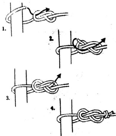
Figure 8 follow through
