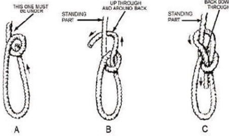
Bowline
