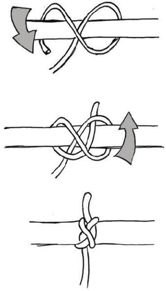
Constrictor Hitch
