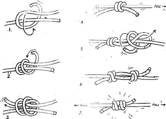
Double Fisherman
