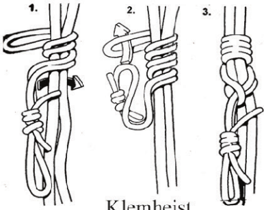
Klemheist
