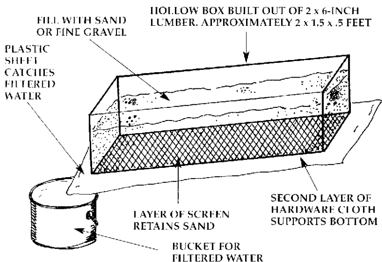
Water filter box.
