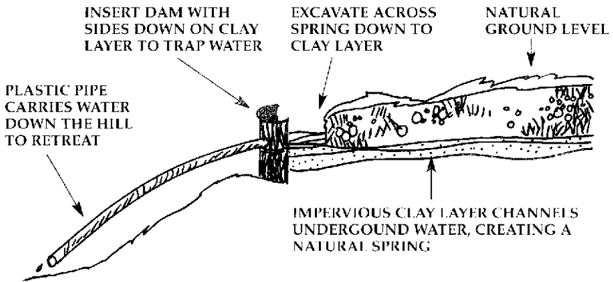
Developing a spring for potable water.
