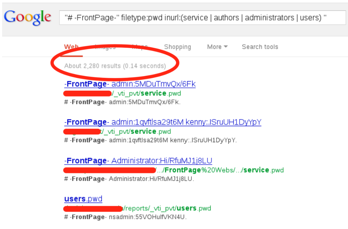
Figure 18 - Using Google to Find Exposed Frontpage Credentials
