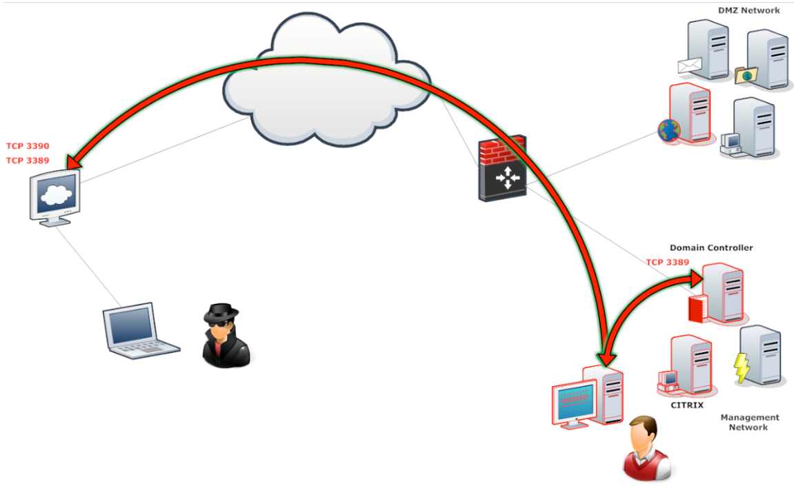
Figure 101 - The Network Has Been Completely Compromised
