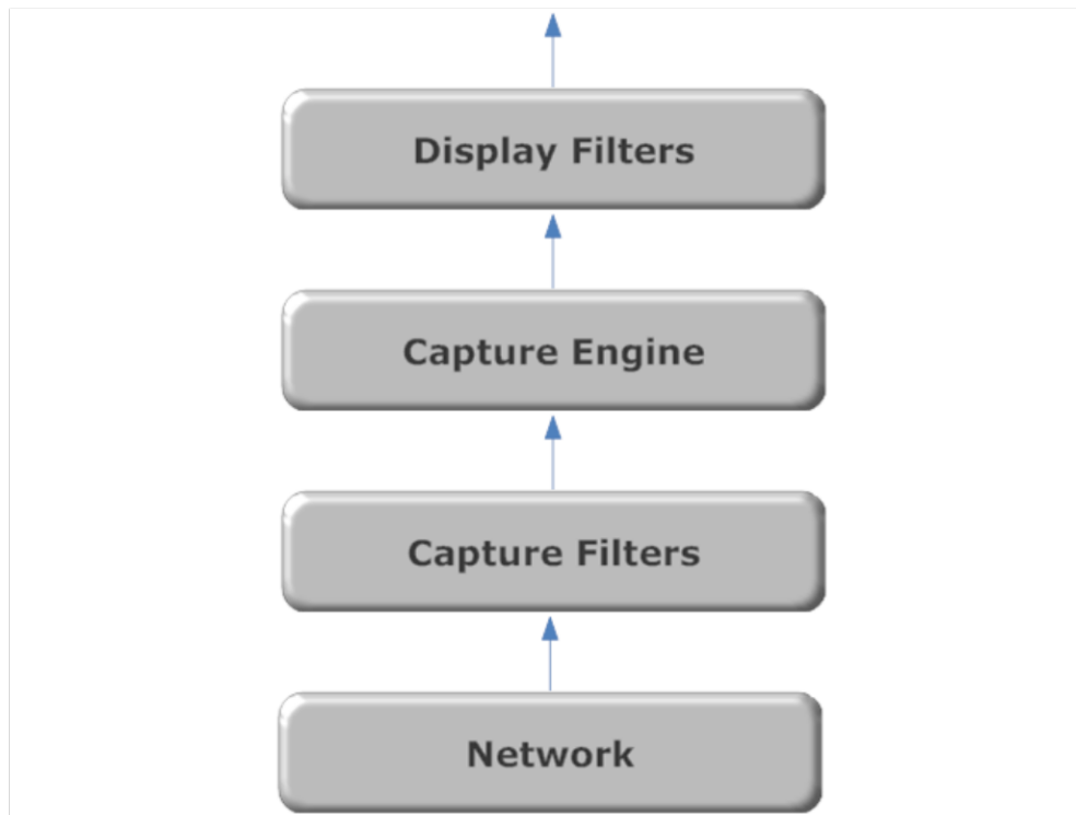
Figure 7 - From the Wire to Wireshark
