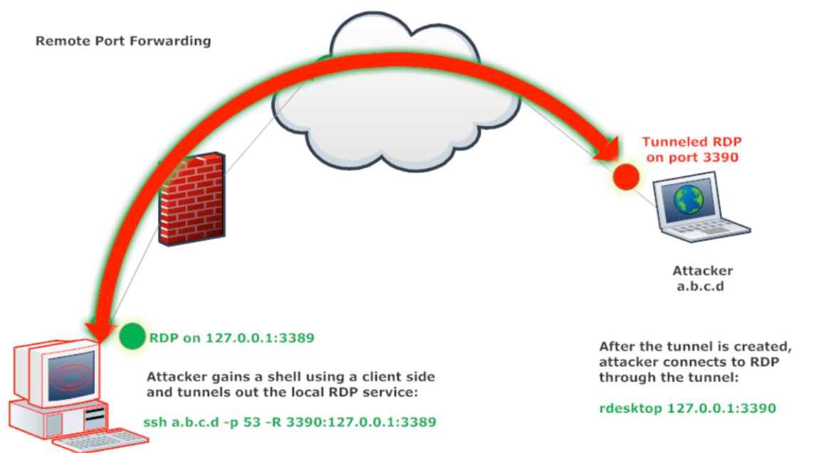
Figure 74 - SSH Remote Port Forwarding
