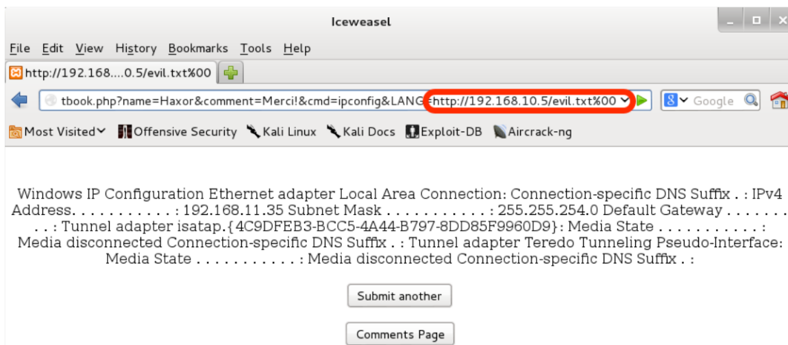
Figure 59 - Exploiting the RFI Vulnerability
