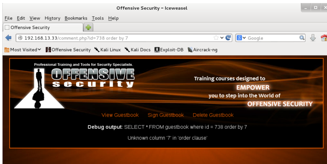
Figure 63 - We Eventually Receive an Error Message
