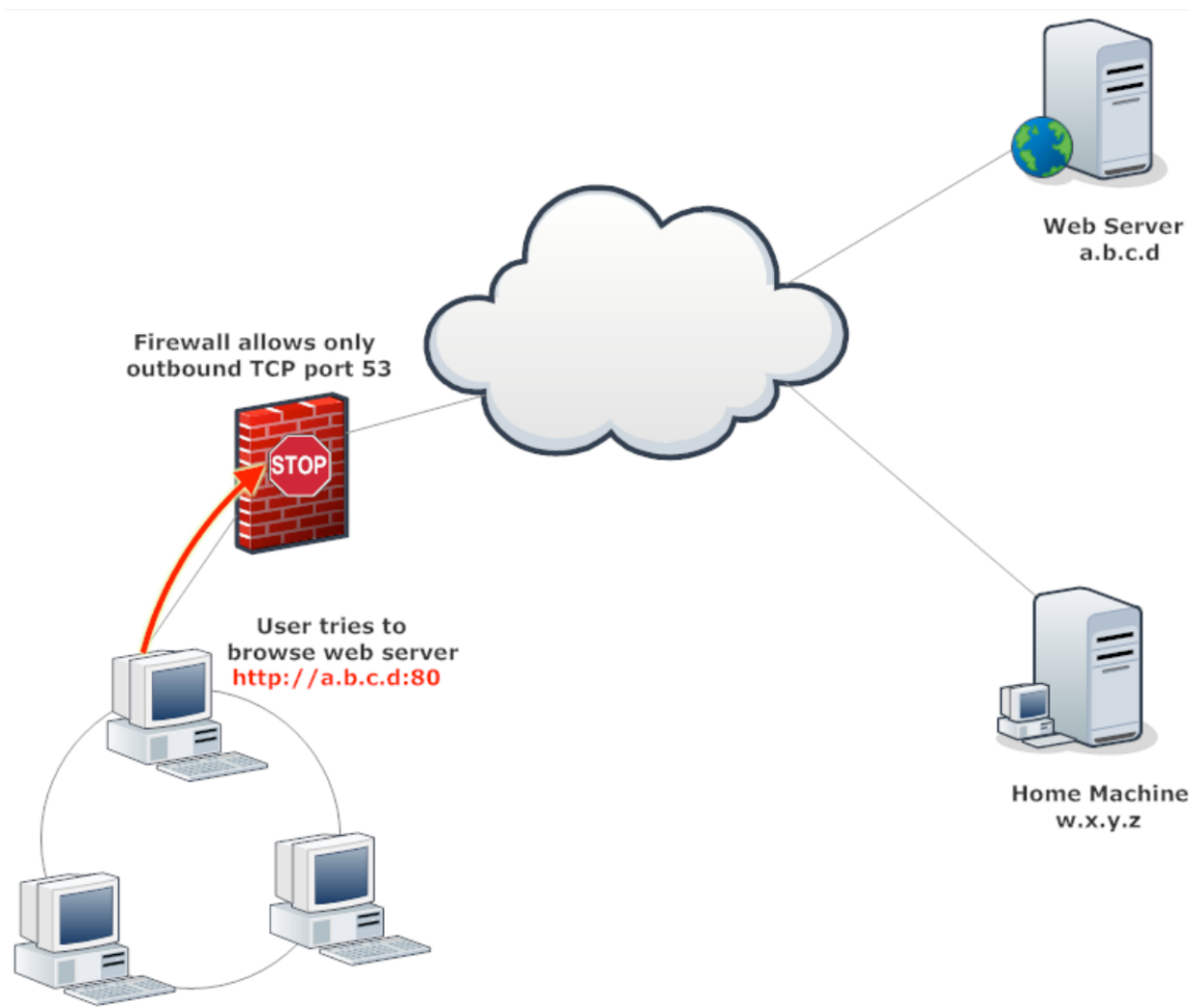
Figure 71 - Outbound Traffic is Only Permitted on TCP Port 53
