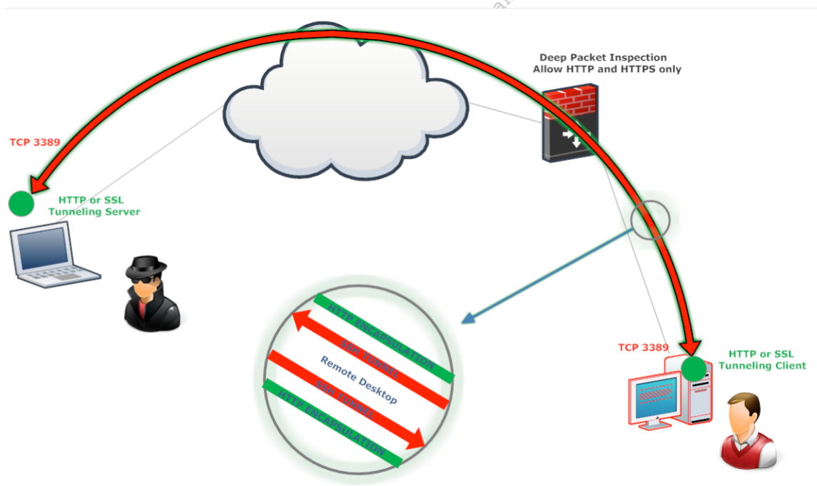
Figure 76 - Circumventing the Deep Packet Inspection System
